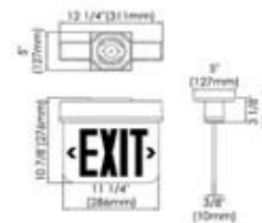
Recessed Mount
