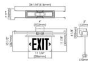
Recessed Mount
