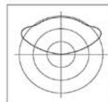
Candela Curve (90 Degree Plane)
