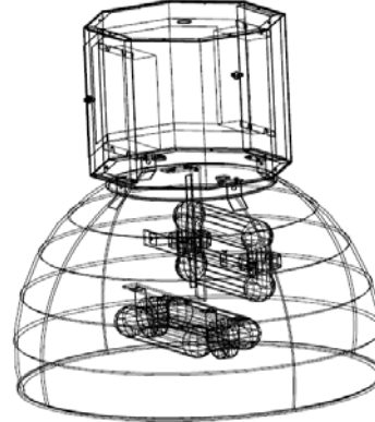
Two Lamp Sylvania Icteron System
